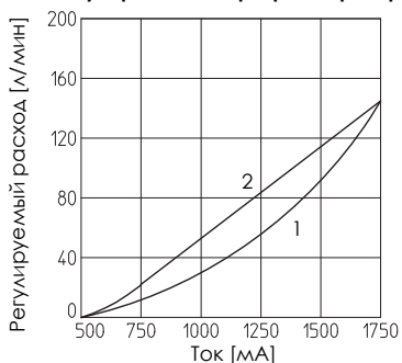
1 = LEQZO-A*-162S4 2 = LEQZO-A*-162L4
