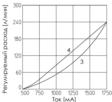
3 = LEQZO-A*-252S4 4 = LEQZO-A*-252L4
