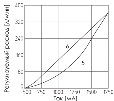
5 = LEQZO-A*-322S4 6 = LEQZO-A*-322L4
